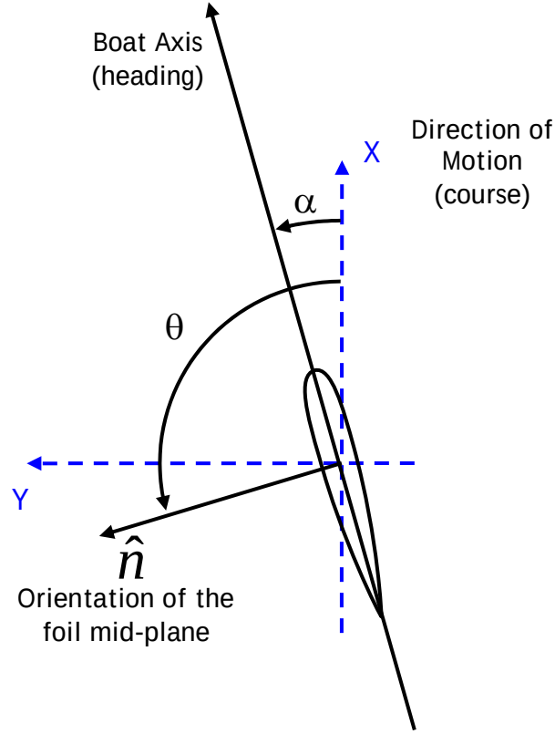
Figure 3: Top view of the geometry in the Z=0 plane.
